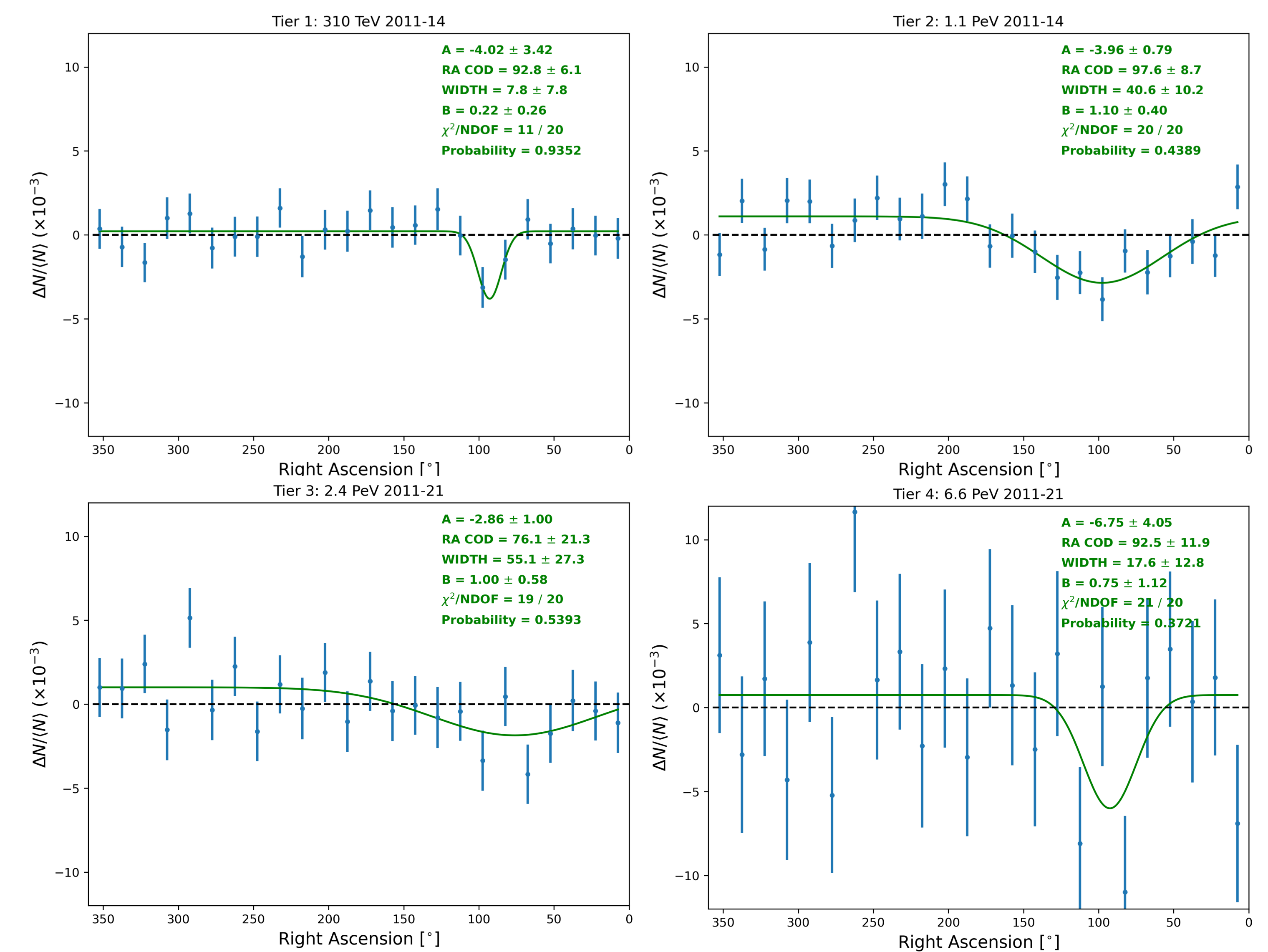
Figure 2: 1D Projections of relative intensity vs right ascension with Gaussian fit per energy band.
